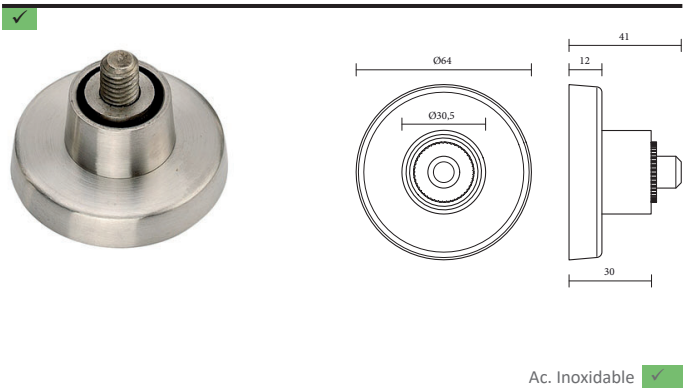
SOPORTE TUBO-PARED
